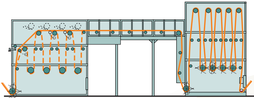
Combined steamer with segments Kombinationsdämpfer in Segmentbauweise
